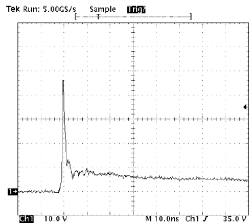
TLP Curve
